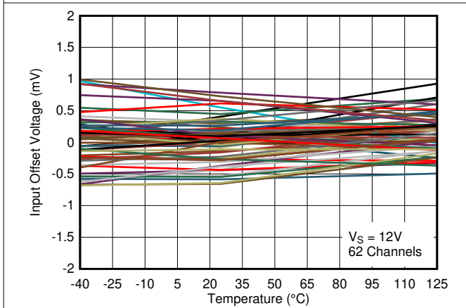
图 3-15. Input Offset Voltage vs. Temperature at 12V
