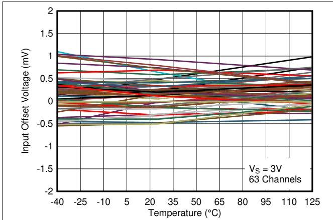
图 3-13. Input Offset Voltage vs. Temperature at 3V
