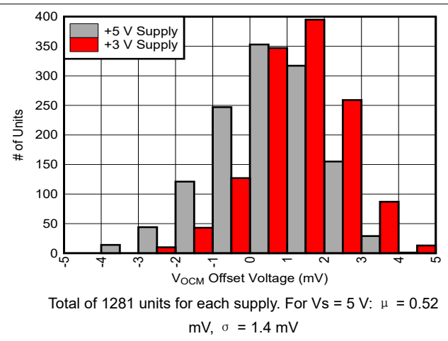
图 7-24. Common-Mode Output Offset from Driven V_{OCM}
