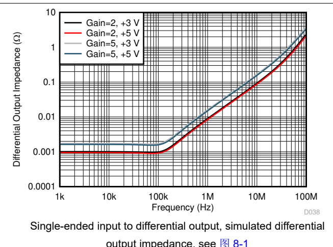
图 7-10. Closed-Loop Output Impedance
