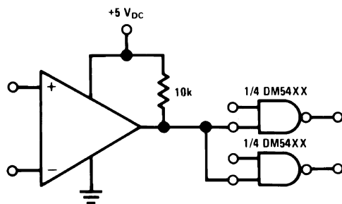
Figure 16. Driving TTL
