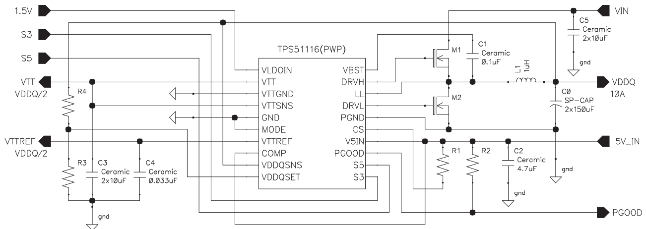
Figure 6. D-CAP™ Mode
