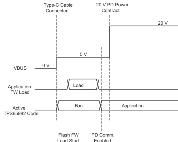
图 10-8. Primary TPS65982 Dead Battery Sequence
