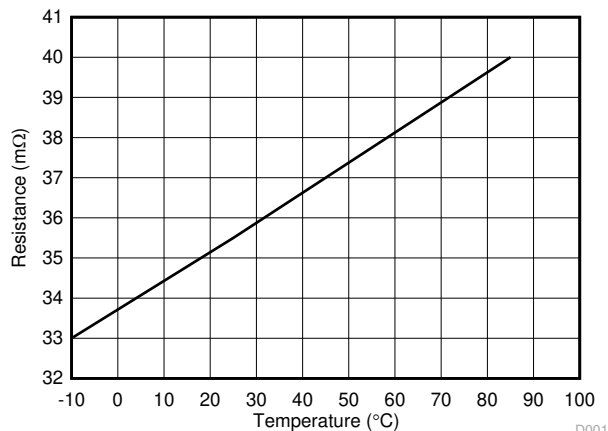
图 7-1. PP_5V0 Switch On-Resistance vs. Temperature
