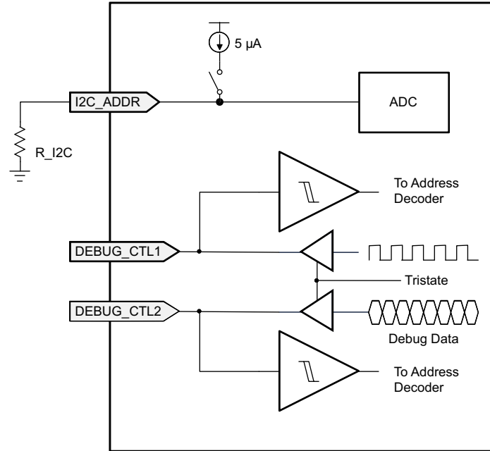
图 9-67. I²C Address Decode
