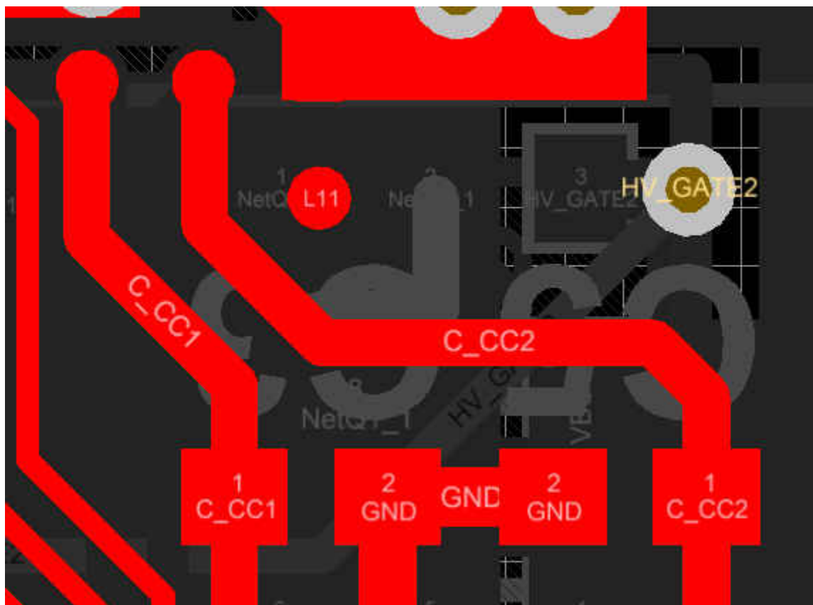
图 12-12. CC1 and CC2 Capacitor Routing
