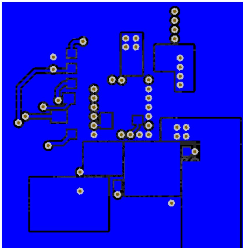
图 12-19. Final Routing (Bottom Layer)
