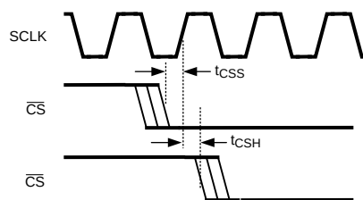
Figure 4. SCLK and \overline{\text{CS}} Timing Parameters
