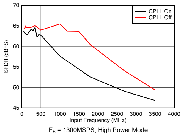
图 5-62. SFDR vs Input Frequency and CPLL
