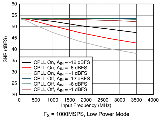
图 5-75. SNR vs Input Frequency, CPLL and Input Amplitude
