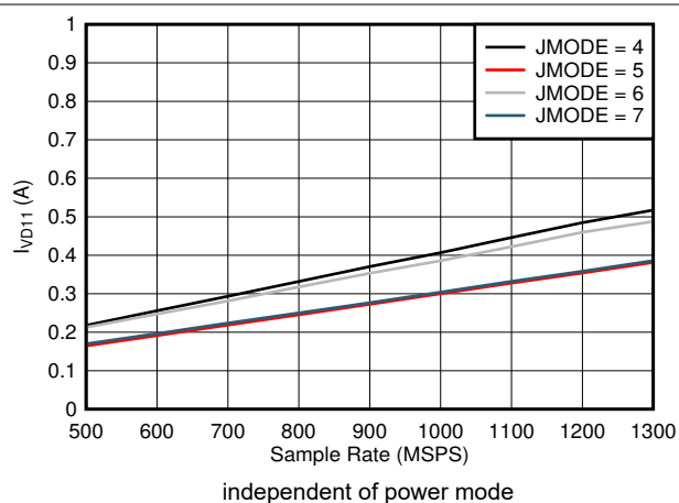
图 5-88. Quad Channel, I_{VD11} vs FS and JMODE 4 - 7
