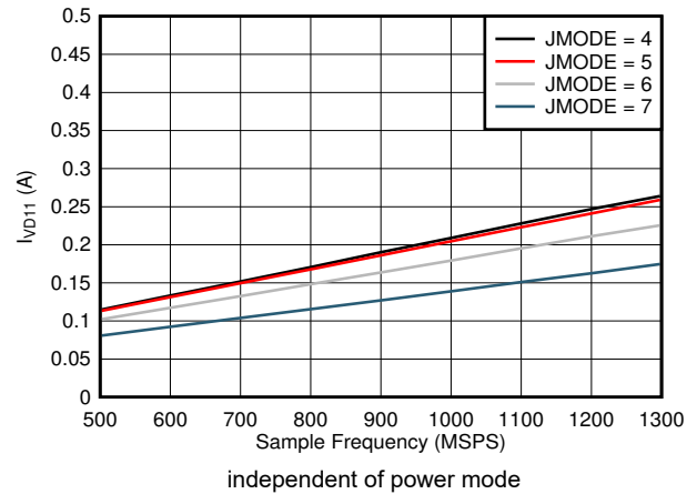
图 5-108. Single Channel, I_{VD11} vs FS and JMODE 4 - 7
