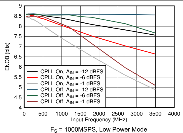
图 5-78. ENOB vs Input Frequency, CPLL and Input Amplitude
