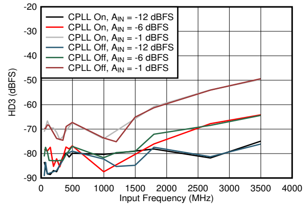
图 5-74. HD3 vs Input Frequency, CPLL and Input Amplitude
