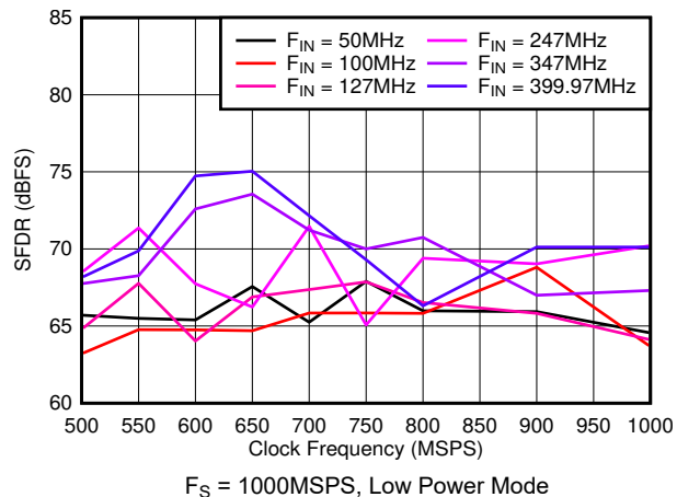
图 5-25. SFDR vs Sample Rate
