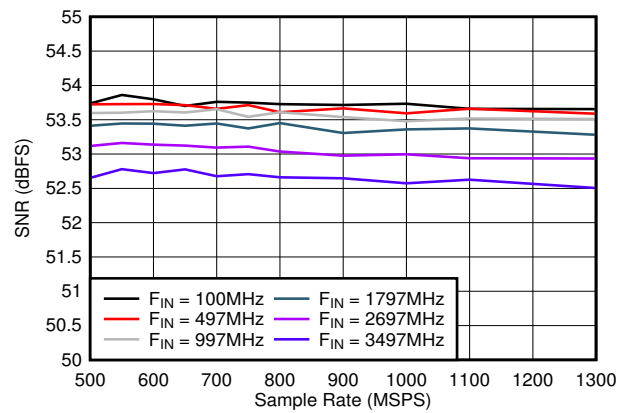
图 5-22. SNR vs Sample Rate
