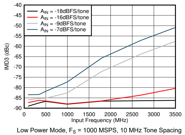
图 5-58. IMD3 vs Input Frequency
