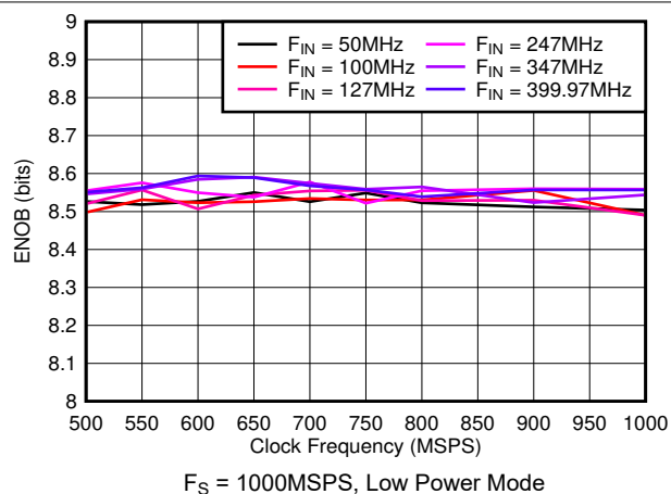
图 5-28. ENOB vs Sample Rate
