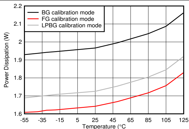
图 5-124. Dual Channel, Power Dissipation vs Temperature
