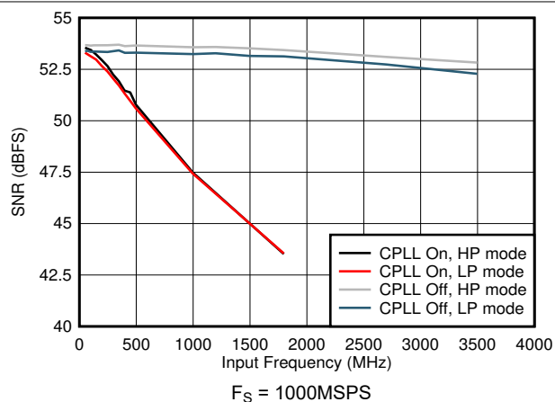
图 5-66. SNR vs Input Frequency and CPLL
