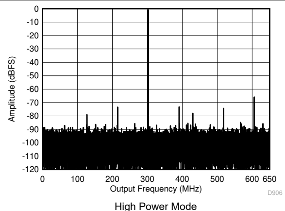
图 5-6. Single Tone FFT at 997 MHz and -1 dBFS
