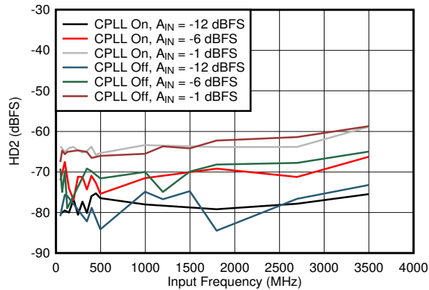
图 5-73. HD2 vs Input Frequency, CPLL and Input Amplitude
