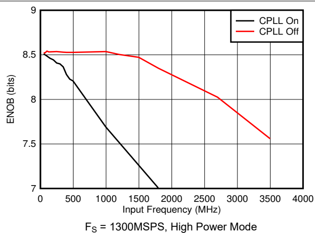
图 5-64. ENOB vs Input Frequency and CPLL
