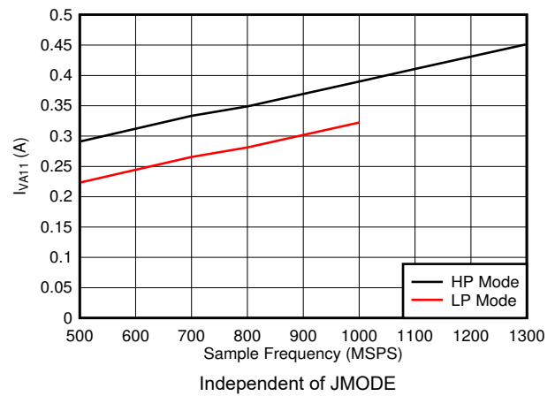
图 5-96. Dual Channel, I_{VA11} vs FS
