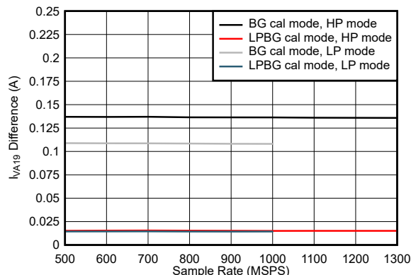
图 5-115. Dual Channel, I_{VA19} Change with Calibration Mode
