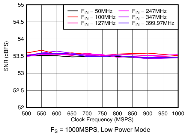
图 5-26. SNR vs Sample Rate
