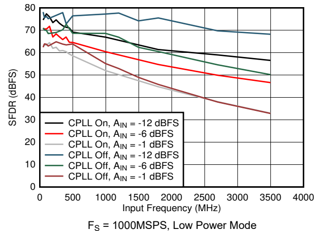
图 5-76. SFDR vs Input Frequency, CPLL and Input Amplitude
