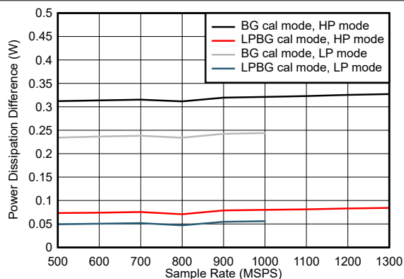
图 5-111. Quad Channel, Power Dissipation Change with Calibration Mode
