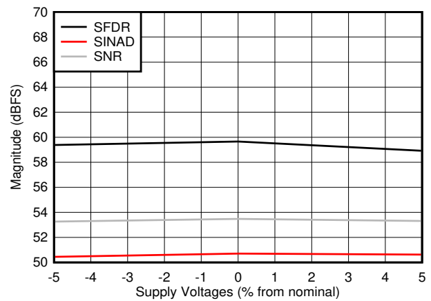
图 5-46. SNR, SFDR and SINAD vs Supply Voltage
