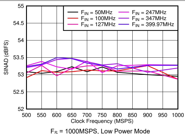
图 5-27. SINAD vs Sample Rate
