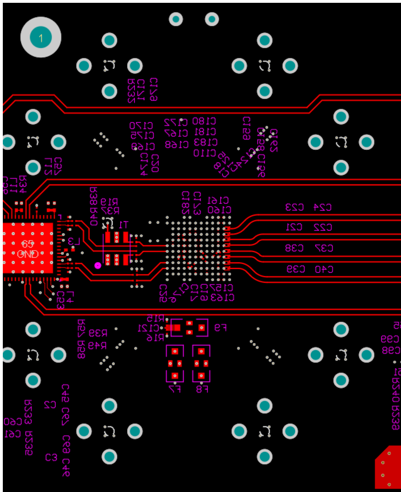
图 7-7. Bottom Layer Routing: CLK±, SYSREF and D[7:4]± Routing
