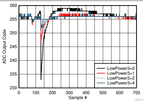
图 6-12. Background Calibration Core Transition In Low Power Mode
