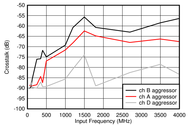
图 5-60. Crosstalk to Channel B vs F_{IN}
