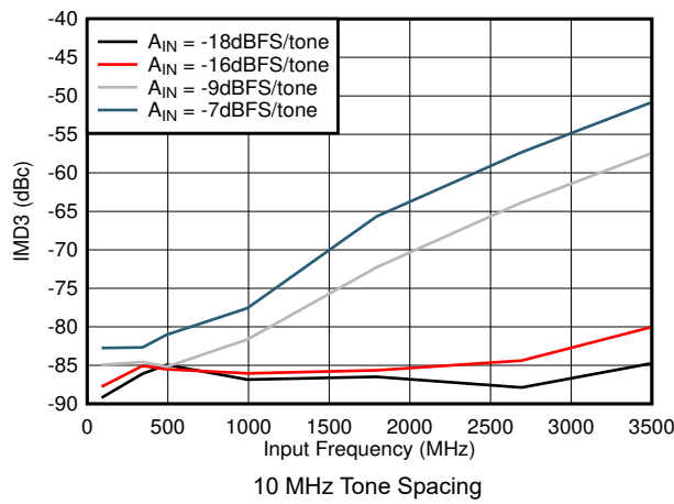
图 5-57. IMD3 vs Input Frequency
