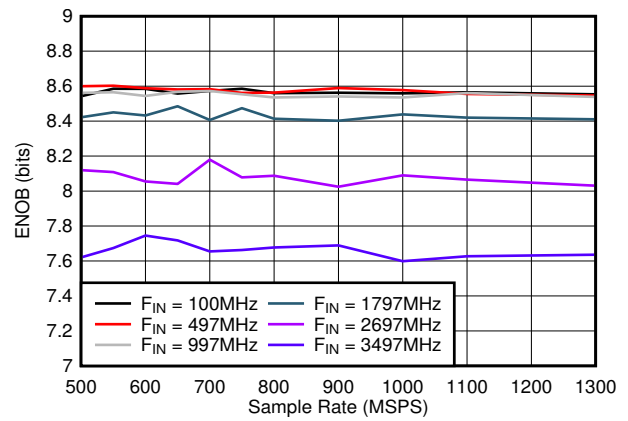
图 5-24. ENOB vs Sample Rate
