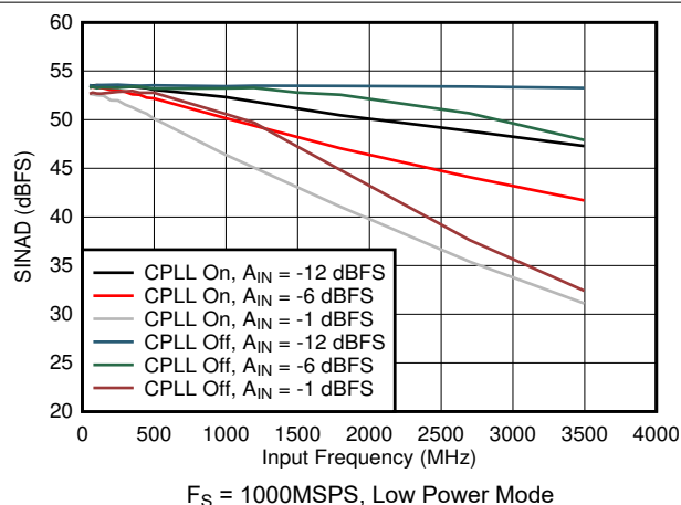
图 5-77. SINAD vs Input Frequency, CPLL and Input Amplitude
