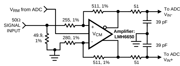
Figure 38. Optional Amplifier Differential Drive Circuit
