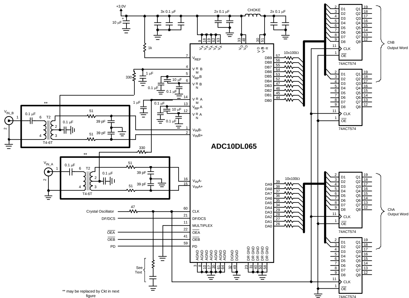
Figure 36. Application Circuit Using Transformer Drive Circuit, Parallel Mode
