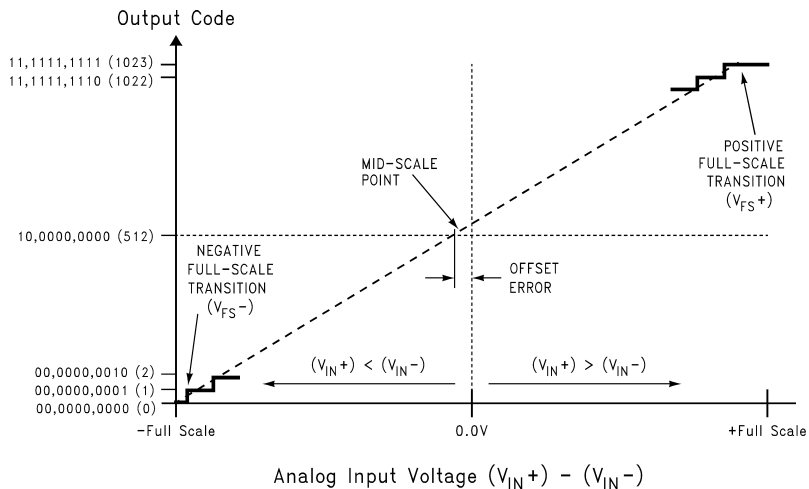
Figure 2. Transfer Characteristic
