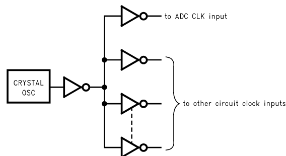
Figure 40. Isolating the ADC Clock from other Circuitry with a Clock Tree
