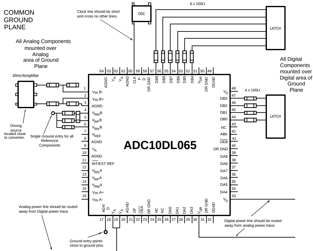
Figure 39. Example of a Suitable Layout
