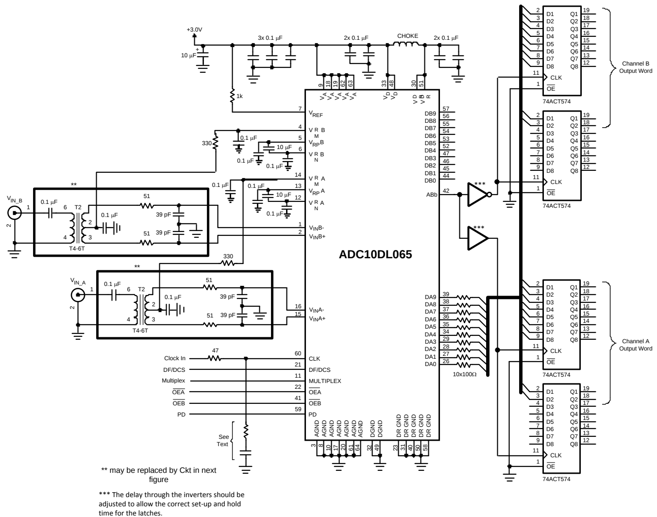
Figure 37. Application Circuit Using Transformer Drive Circuit, Multiplex Mode
