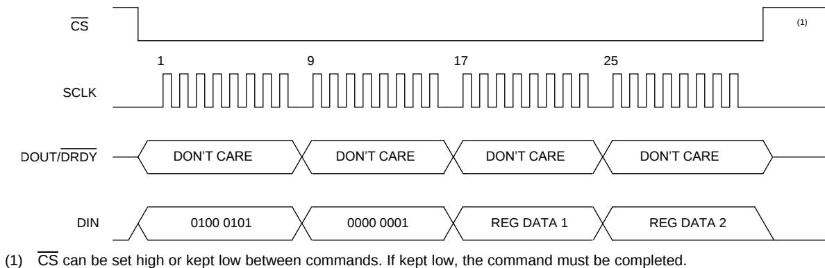
图 89. Write Register Sequence
