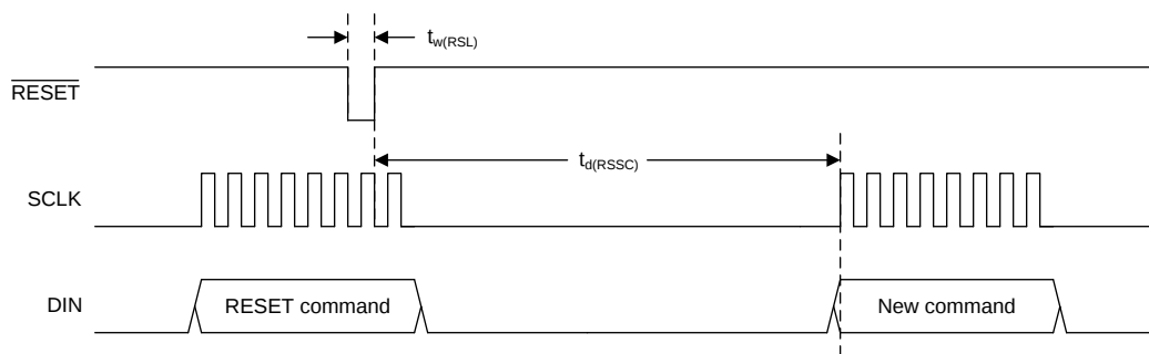
图 3. RESET Pin and RESET Command Timing Requirements
