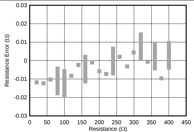
图 115. Measured Resistance Error vs Equivalent RTD Resistance
