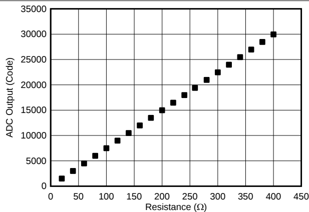
图 114. ADC Output Code vs Equivalent RTD Resistance
