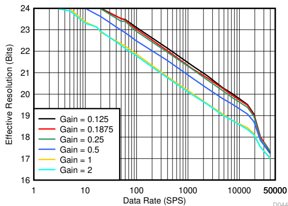
图 8-3. Effective Resolution vs Data Rate
