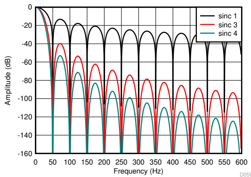
图 9-11. Sinc Filter Frequency Response (50 SPS)
