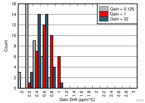
图 7-19. Gain Drift Distribution
