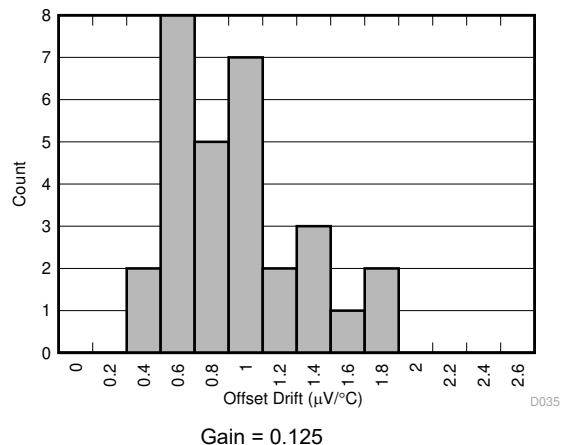
图 7-13. Offset Error Drift Distribution
