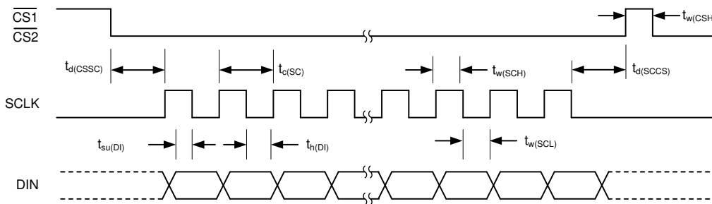
图 7-1. Serial Interface Timing Requirements
