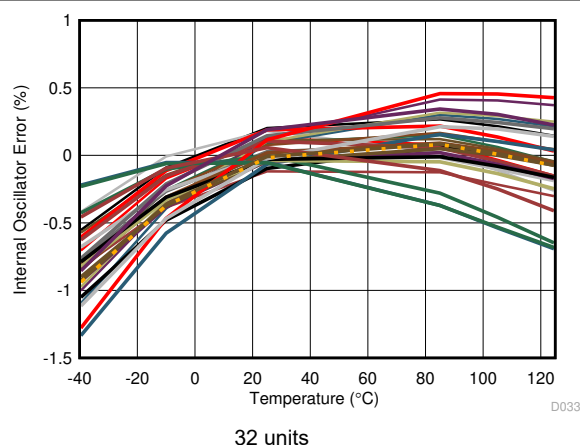
图 7-25. Oscillator Frequency Error vs Temperature
