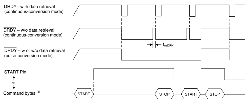
图 9-19. \overline{\text{DRDY}} Operation
