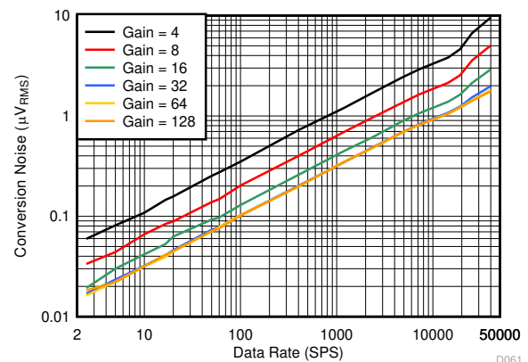
Gain = 4 to 128, V_{\text{REF}} = 2.5\text{ V} , sinc3 filter (sinc5 filter for f_{\text{DATA}} \geq 14.4\text{ kSPS} )
