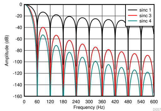
图 9-12. Sinc Filter Frequency Response (60 SPS)
