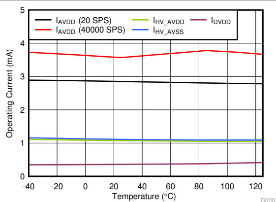
图 7-30. Operating Current vs Temperature
