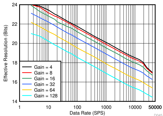
图 8-4. Effective Resolution vs Data Rate
