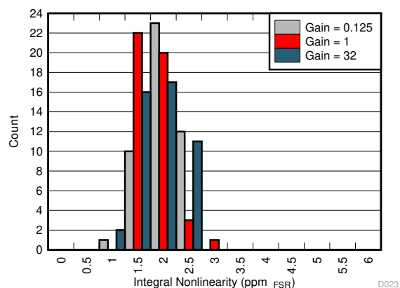
图 7-12. Nonlinearity Distribution
