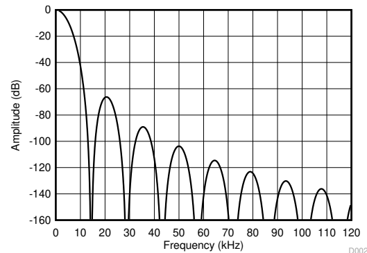
图 9-8. Sinc5 Filter Frequency Response (14.4 kSPS)
