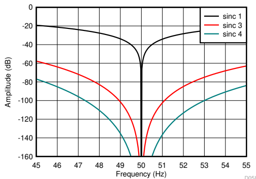
图 9-13. Sinc Filter Frequency Response (50 SPS)
