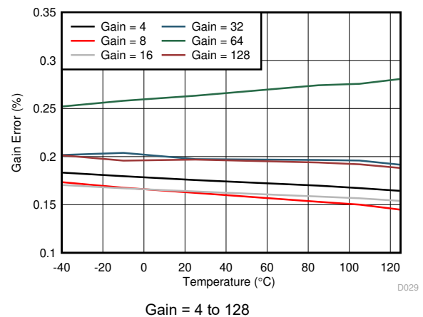
图 7-21. Gain Error vs Temperature
