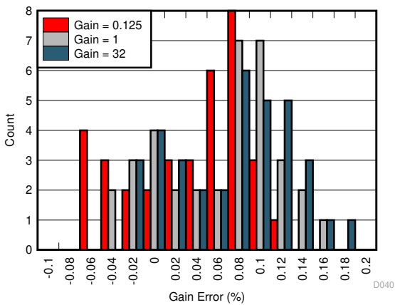
图 7-18. Gain Error Distribution
