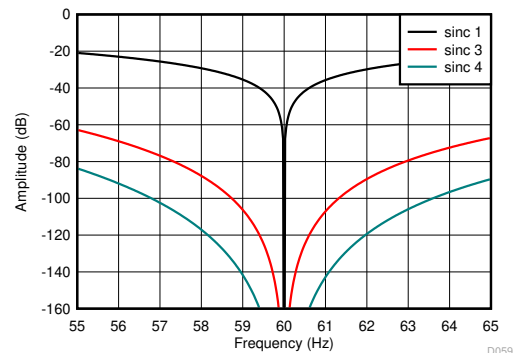
图 9-14. Sinc Filter Frequency Response (60 SPS)
