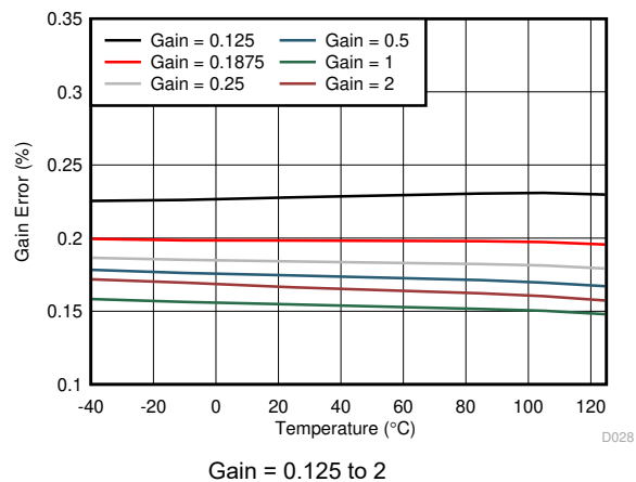
图 7-20. Gain Error vs Temperature
