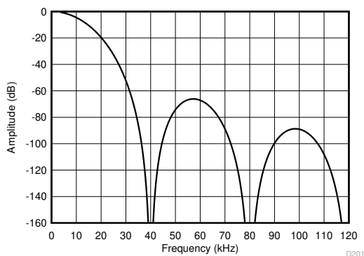
图 9-7. Sinc5 Filter Frequency Response (40 kSPS)
