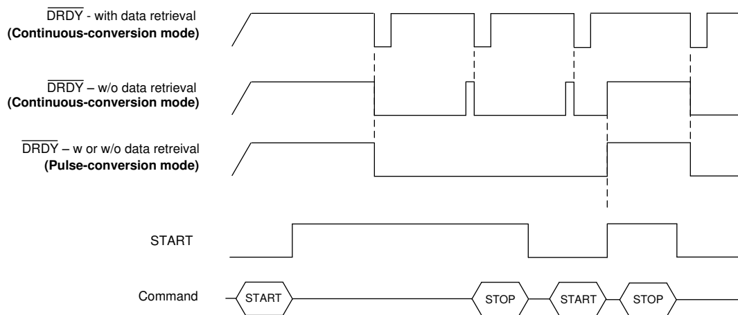
图 79. \overline{DRDY} Operation
