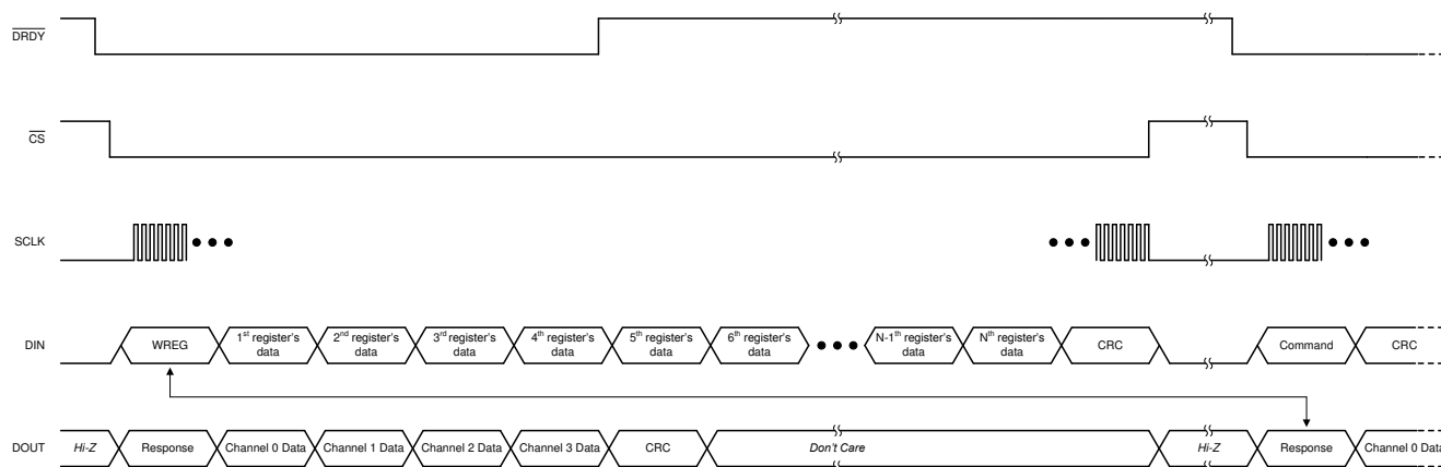
图 8-21. Writing Registers
