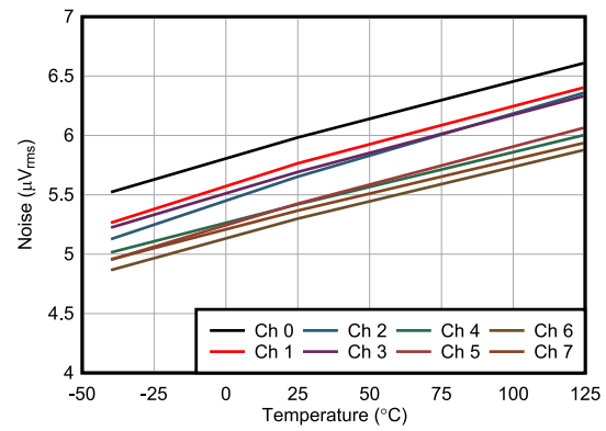
图 6-17. Noise vs Temperature
