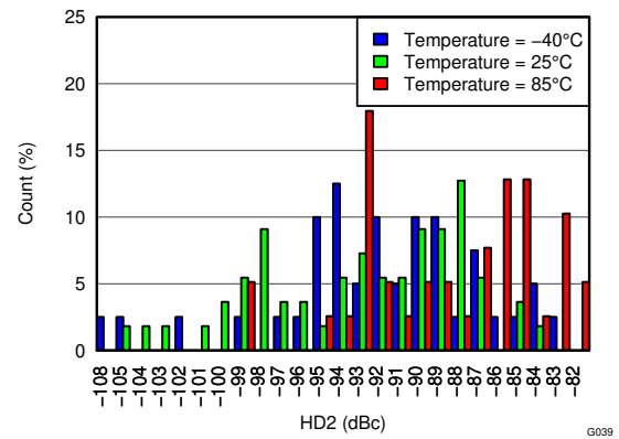
图 6-13. HD2 Distribution over Multiple Devices
