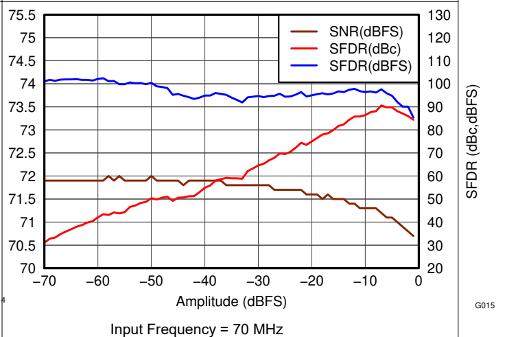
图 6-17. Performance vs Input Amplitude
