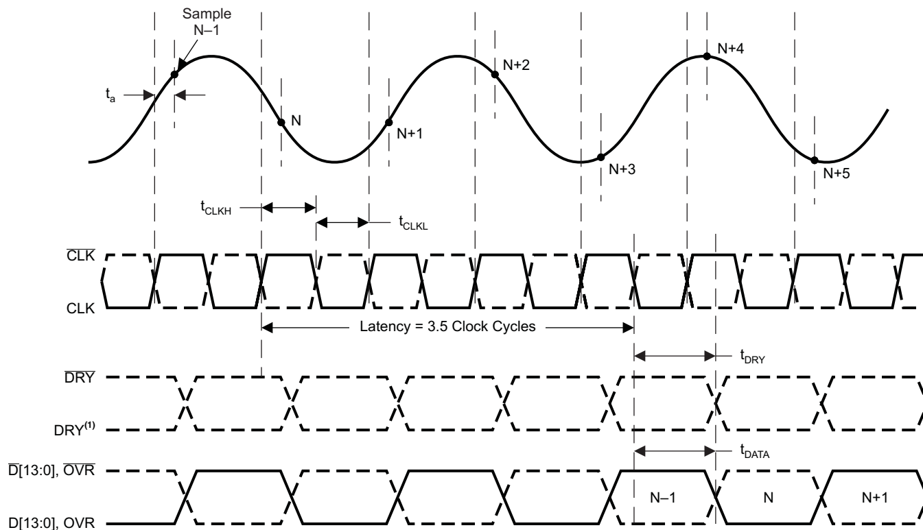
Figure 1. Timing Diagram
