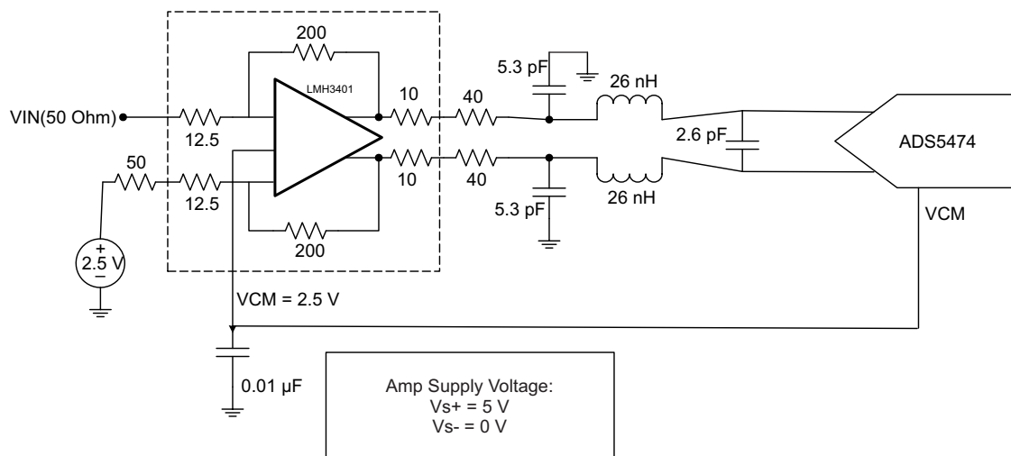
Figure 43. Application Diagram
