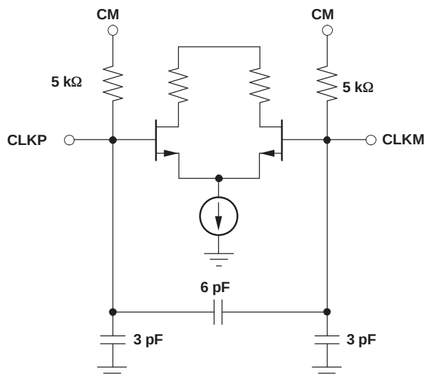
Figure 45. Clock Inputs
