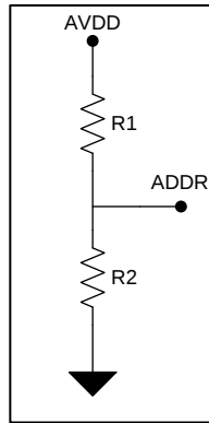
图 45. External Resistor Connection Diagram for ADDR Pin
