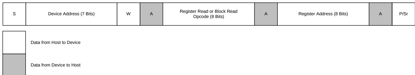
图 49. Setting Register Address for Reading Registers
