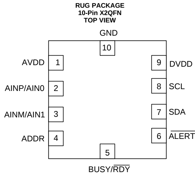
Pin Functions
