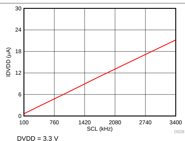
图 70. I_{DVDD} in Manual Mode with SCL
