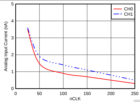
Input Voltage = 1.5 V Stop Burst Mode With Low Power Oscillator
