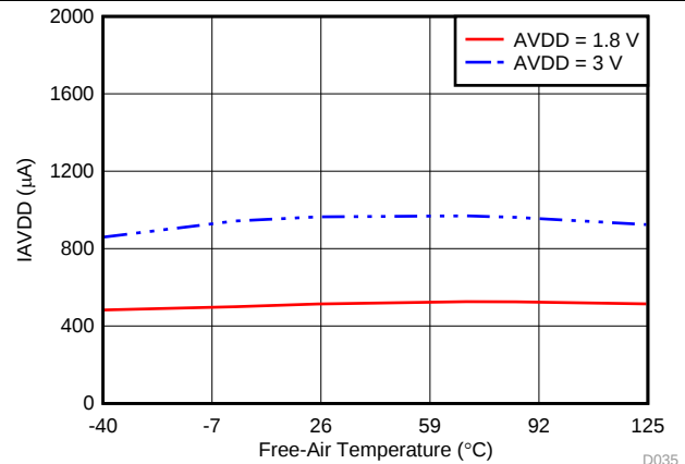
Stop Burst Mode nCLK = 25 With High Speed Oscillator
