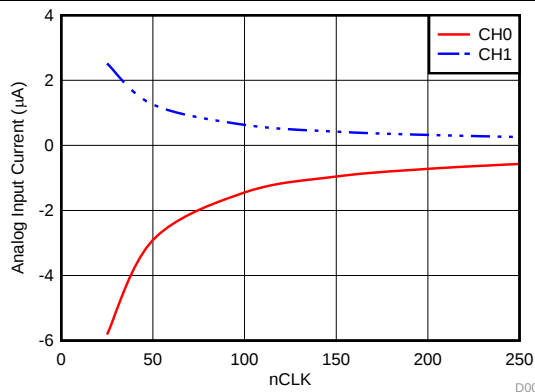
Input Voltage = 1.5 V Stop Burst Mode With High Speed Oscillator
