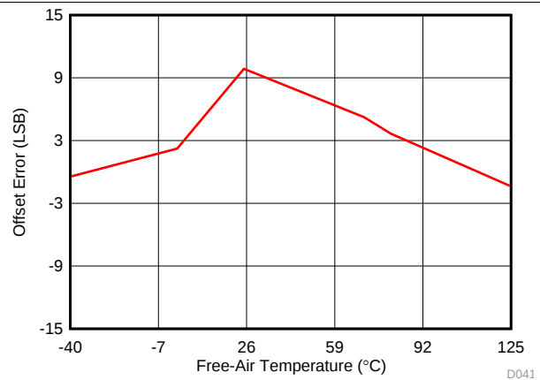
图 35. Offset Error in High Precision Mode with Temperature
