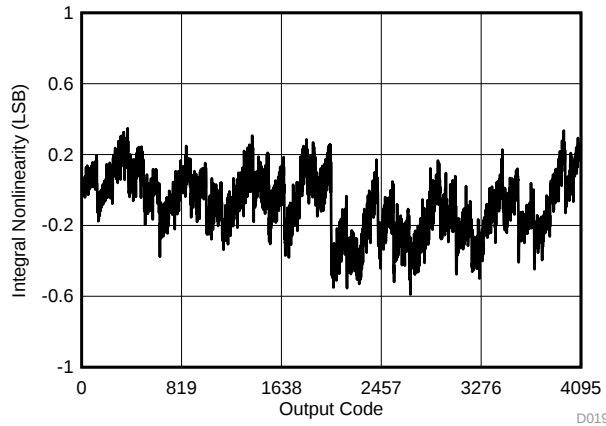
图 19. Typical INL in Manual Mode
