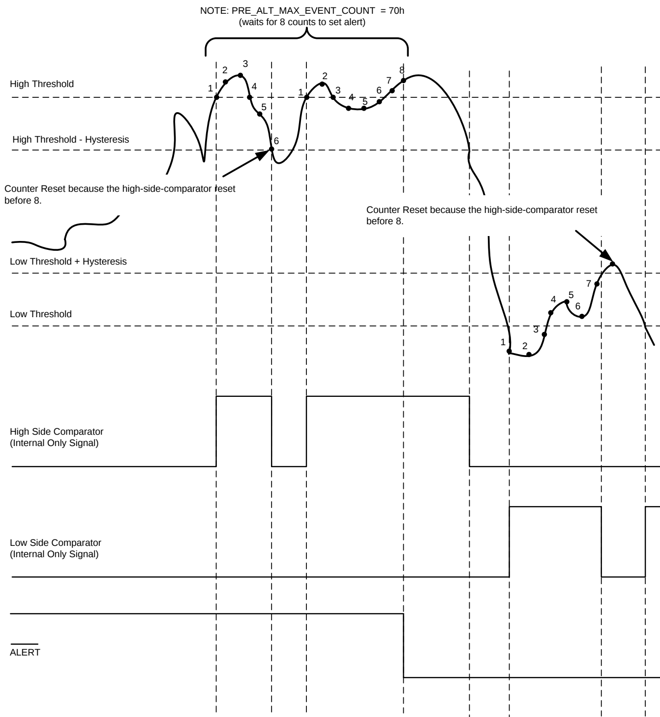
图 48. Thresholds, Hysteresis and Event Counter for Digital Window Comparator
