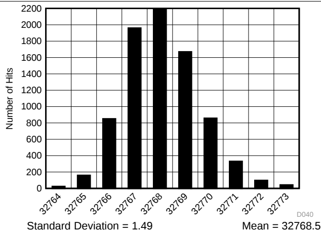
图 34. Typical DC Code Spread in High Precision Mode
