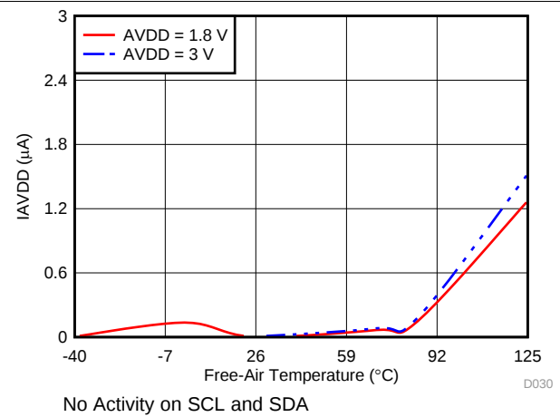
图 28. Static I_{AVDD} in Manual Mode with Temperature
