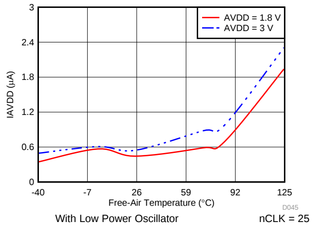
图 37. I_{AVDD} in High Precision Mode with Temperature
