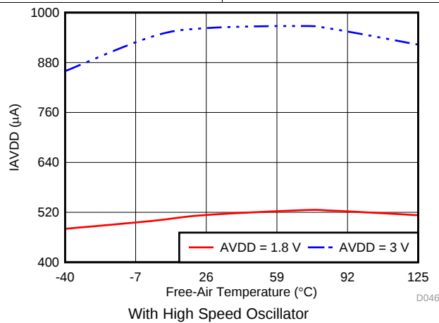
图 38. I_{AVDD} in High Precision Mode with Temperature
