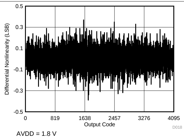
图 18. Typical DNL in Manual Mode
