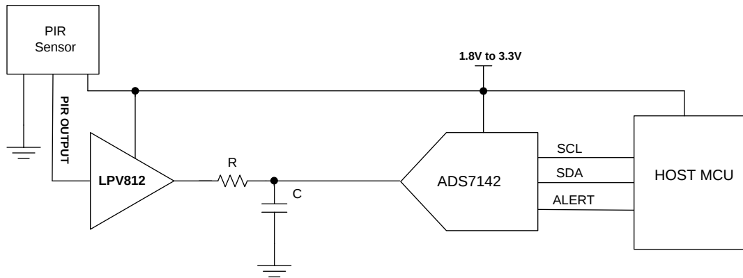
图 119. PIR Sensor with ADS7142
