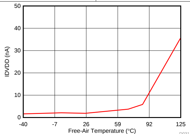
图 27. I_{DVDD} in Manual Mode with SCL
