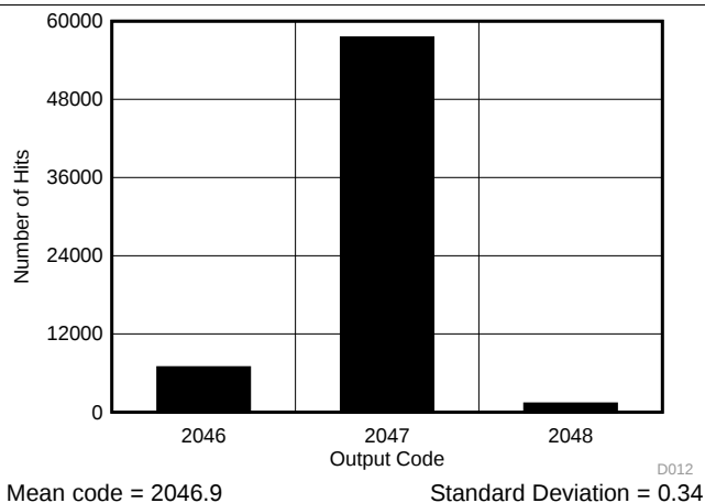
图 12. Typical DC Code Spread in Manual Mode
