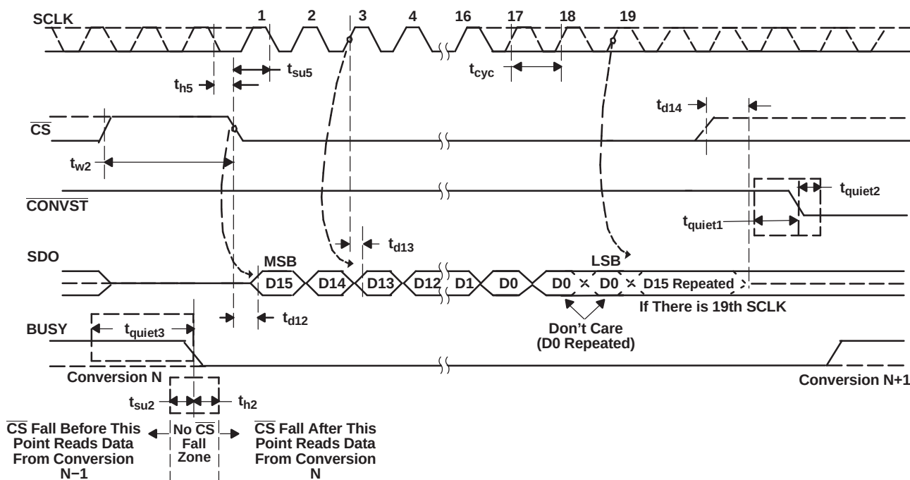
Figure 45. Read Frame Controlled via \overline{\text{CS}} (FS = 1)
