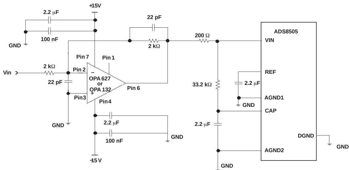
Figure 27. Typical Driving Circuit ( \pm 10\text{ V} , No Trim)
