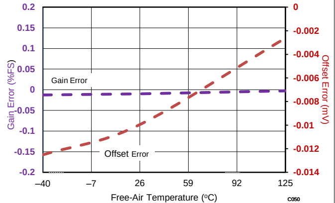
Figure 66. Offset and Gain vs Temperature (AUX Channel)
