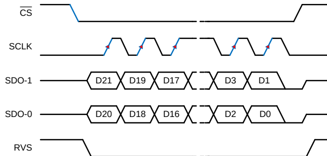
Figure 68. SPI-00-D-EDL Protocol
