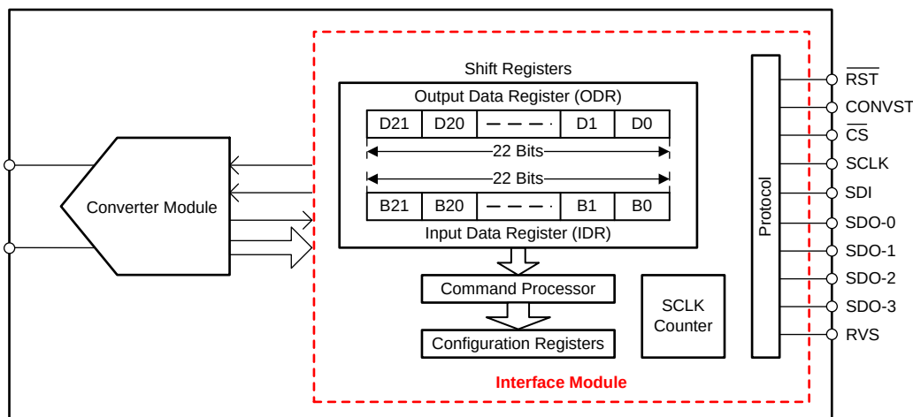
Figure 37. Interface Module
