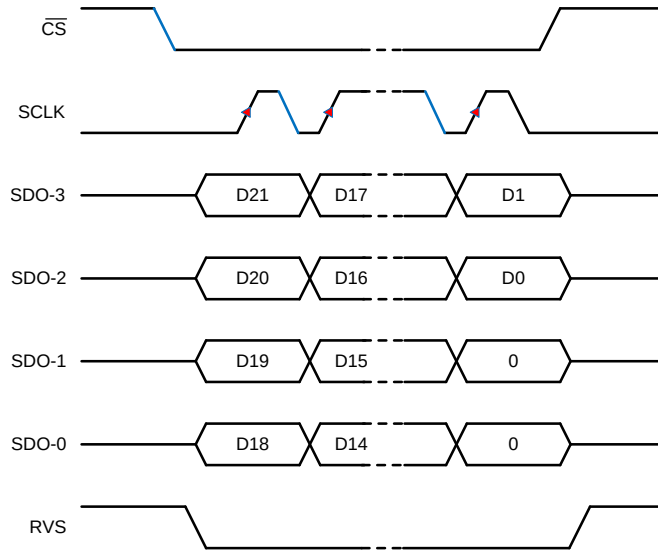
Figure 64. SPI-00-Q Protocol
