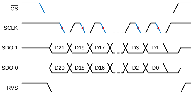
Figure 69. SPI-10-D-EDL Protocol
