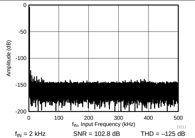
Figure 21. Typical FFT
