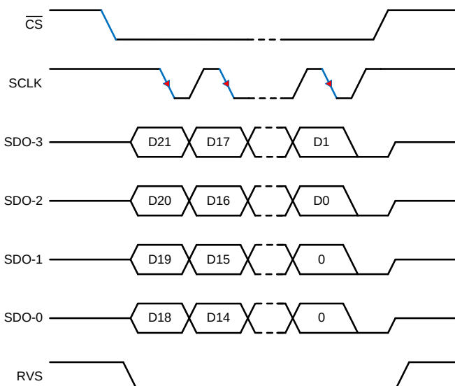
Figure 71. SPI-10-Q-EDL Protocol
