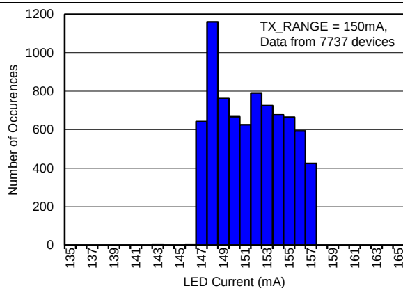
Figure 48. LED Current with Tx DAC Setting = 255 (150 mA)
