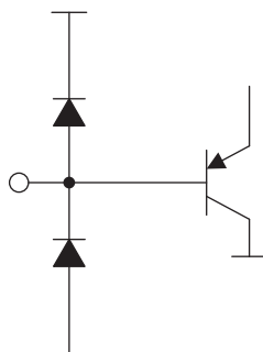
Figure 93. Equivalent Circuits of V_{\text{CNTLP/M}}
