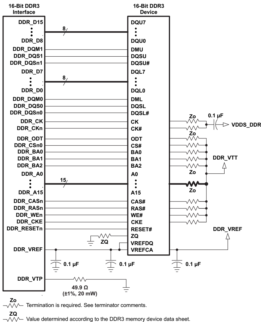
图 7-47. 16-Bit DDR3 Interface Using One 16-Bit DDR3 Device with V_{\Pi} Termination
