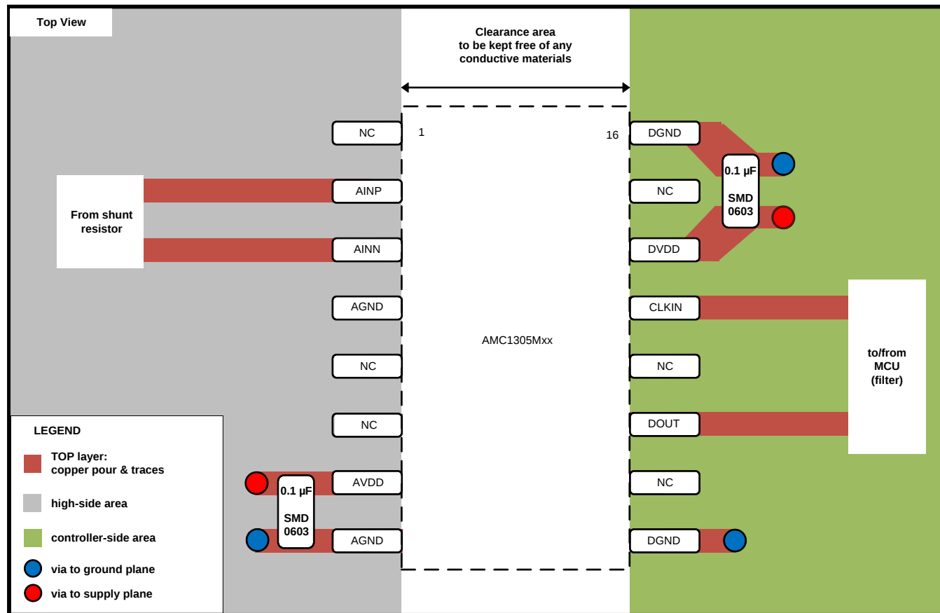
Figure 59. Recommended Layout of the AMC1305Mxx
