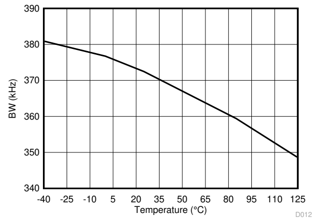
图 5-12. Output Bandwidth vs Temperature
