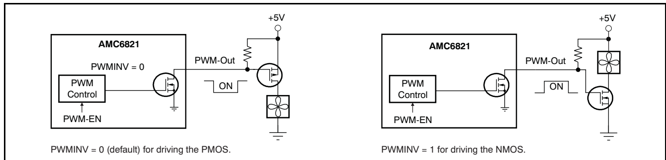
Figure 15. PWM Output
