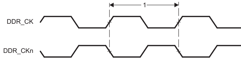
图 7-46. DDR3 Memory Interface Clock Timing
