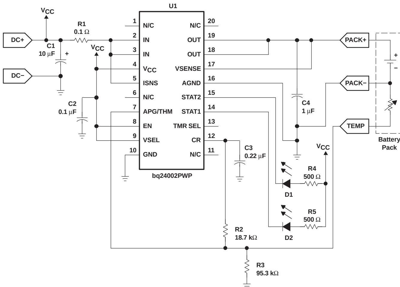
Figure 13. Li-Ion/Li-Pol Charger
