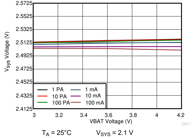
图 10-23. 2.1 V SYS Line Regulation
