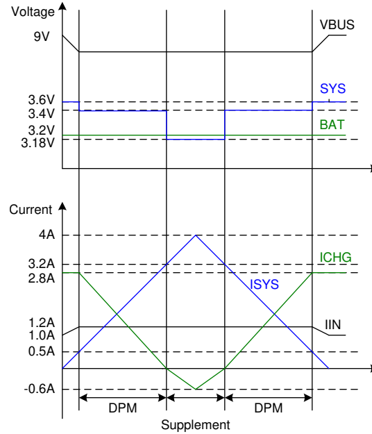
图 8-8. DPM Response
