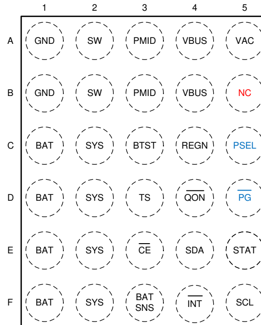
图 6-1. BQ25600 YFF Package 30-Pin WCSP Top View
