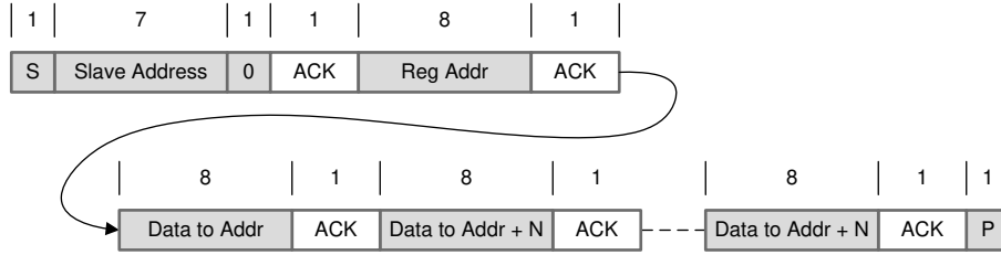
图 9-18. Multi-Write
