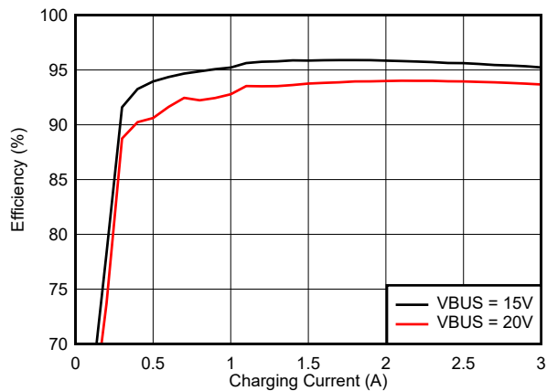
图 7-4. 2s Battery Charge Efficiency, 1.5 MHz
