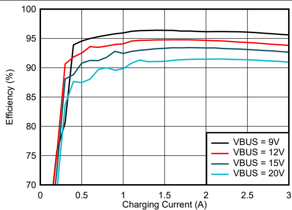
图 7-2. 1s Battery Charge Efficiency, 1.5 MHz
