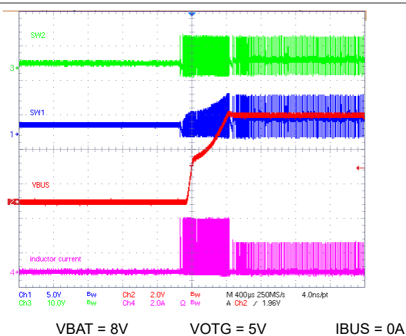
图 9-5. OTG Startup at No Load
