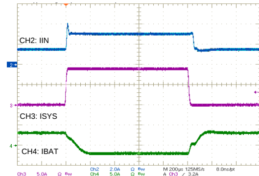
图 57. System Regulation in Buck Boost Mode
