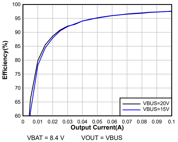
图 8-12. PTM Mode Light Load System Efficiency
