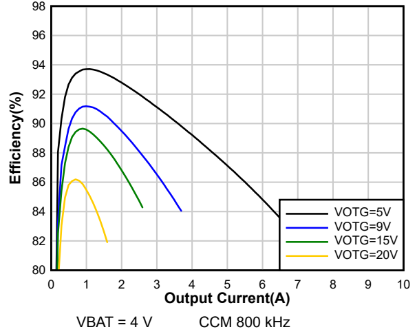
图 8-8. OTG Efficiency with 1S Battery
