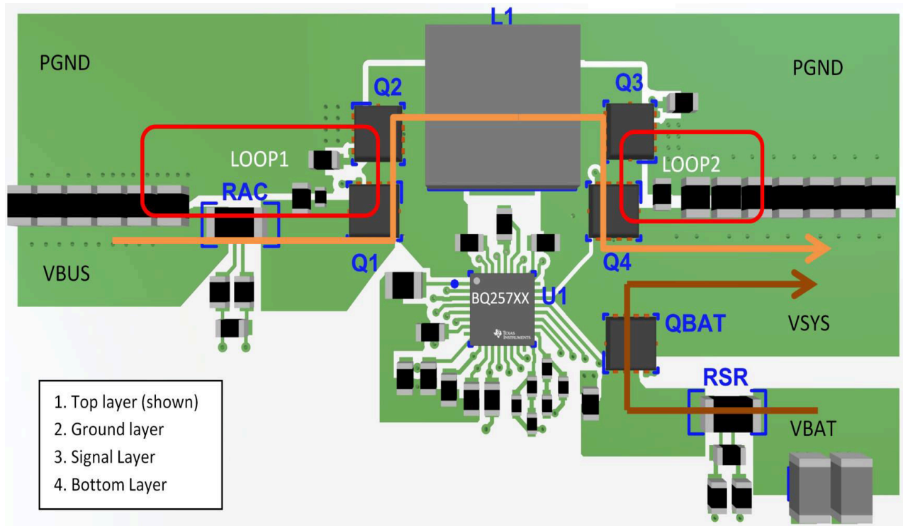
图 12-1. Buck-Boost Charger Layout Reference Example Top View
