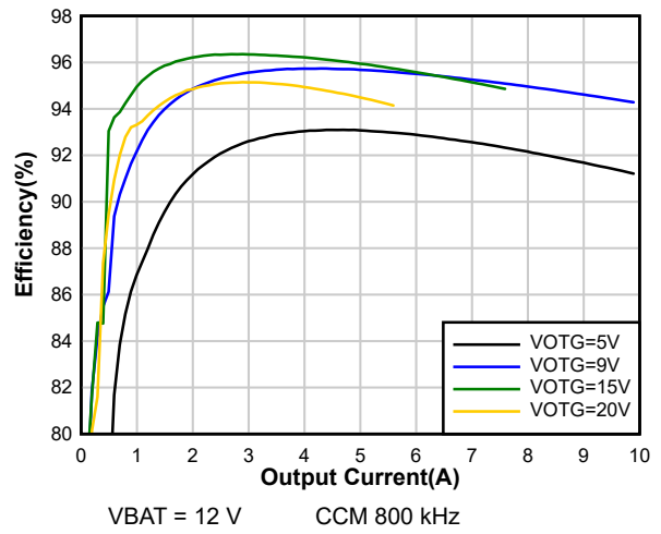
图 8-10. OTG Efficiency with 3S Battery
