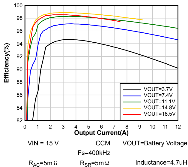
图 8-3. Charge Efficiency
