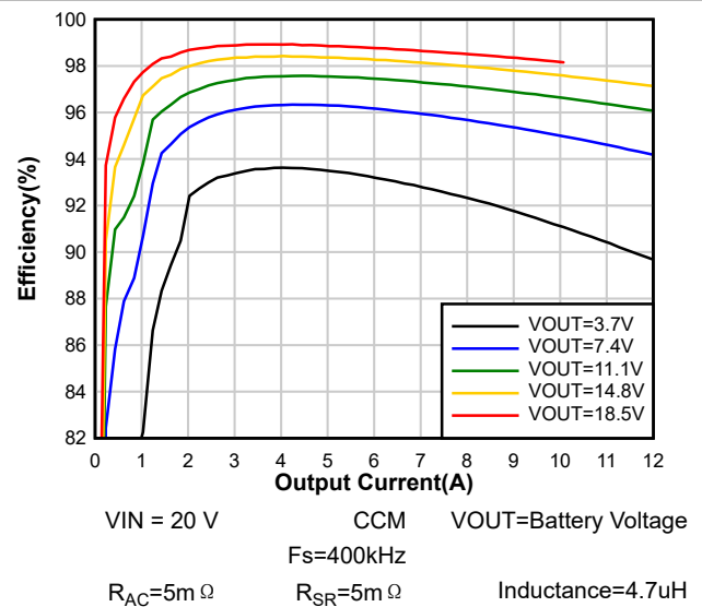
图 8-4. Charge Efficiency
