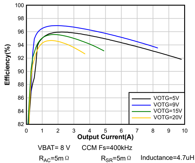
图 8-7. OTG Efficiency with 2S Battery
