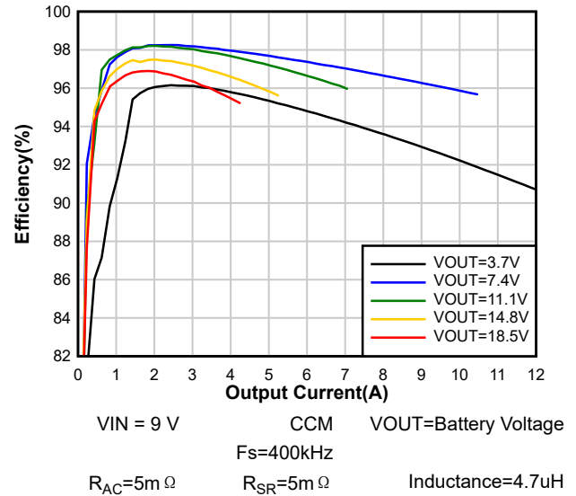
图 8-2. Charge Efficiency
