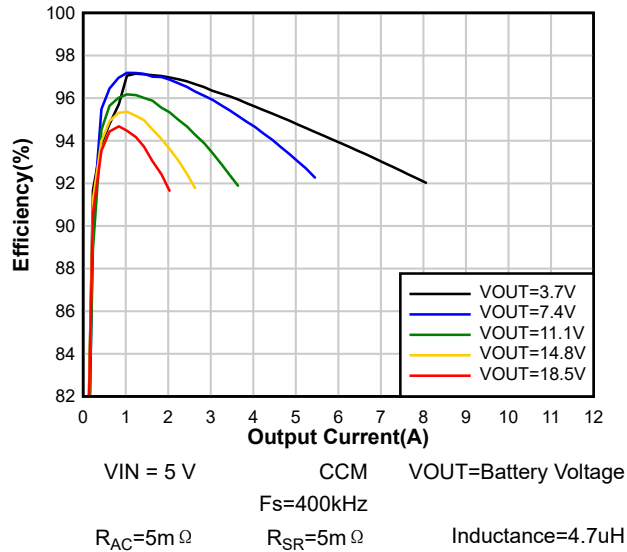
图 8-1. Charge Efficiency
