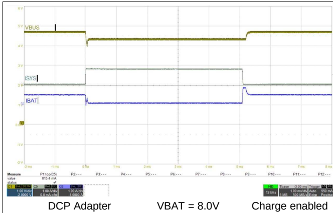
图 86. VINDPM Transient Response
