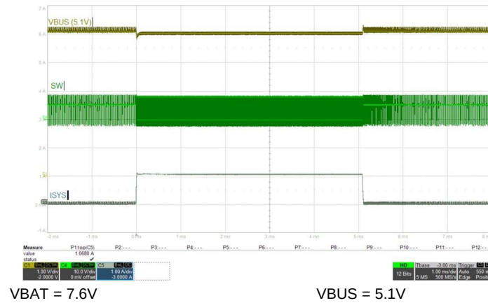
图 88. Buck Mode (OTG) Load Transient Response
