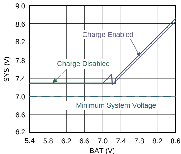
图 17. System Voltage vs. Battery Voltage
