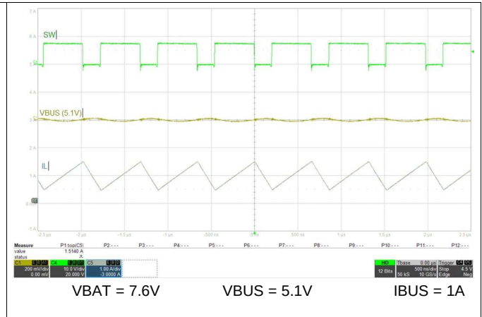
图 81. Buck Mode (OTG) PWM Switching
