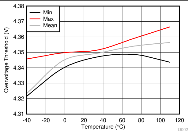
图 7-2. BQ294502 Overvoltage Threshold (OVT) vs Temperature
