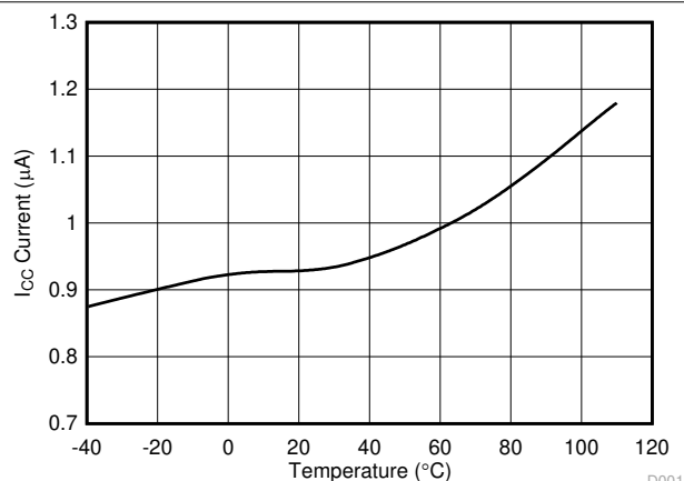
图 7-1. I_{CC} Current Consumption vs Temperature
