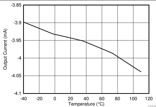
图 7-4. Output Current I_{OUT} vs Temperature
