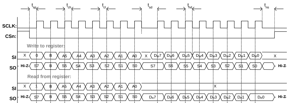
Figure 15: Configuration Registers Write and Read Operations
