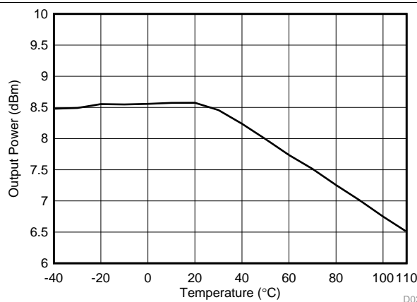
Figure 5-44. TX Bluetooth low energy Maximum Output Power vs Temperature, 2440 MHz
