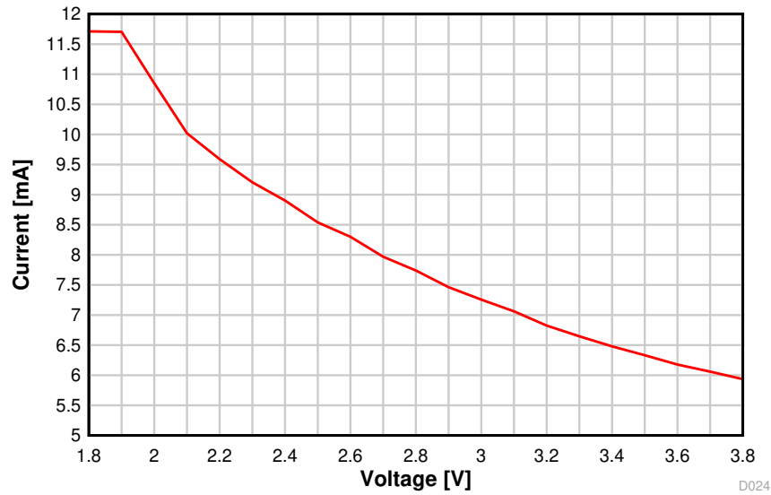
图 8-20. TX Current vs. Supply Voltage (VDD5) (BLE 1 Mbps, 2.44 GHz)
