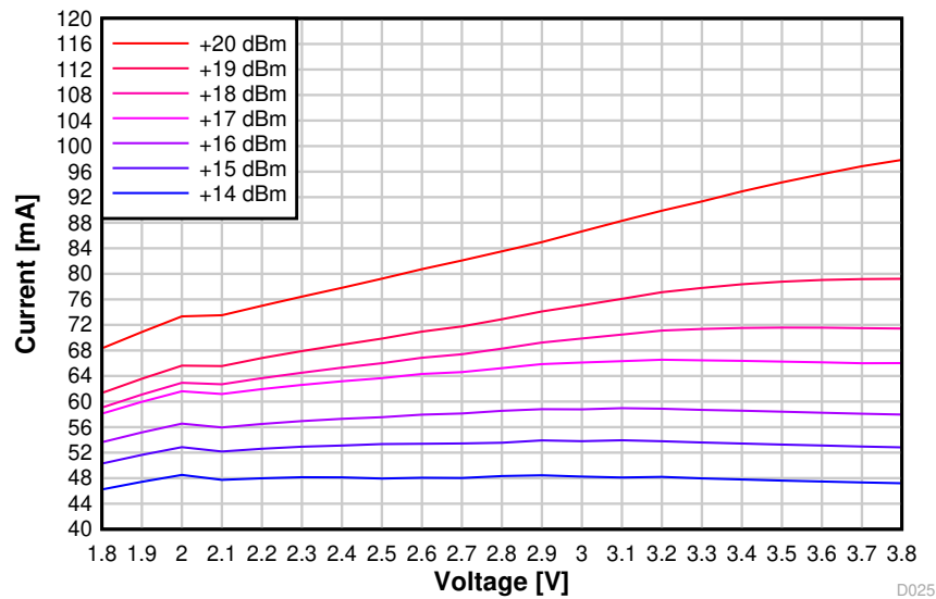
图 8-21. TX Current vs. Supply Voltage (VDD5) (BLE 1 Mbps, 2.44 GHz, +20 dBm PA)
