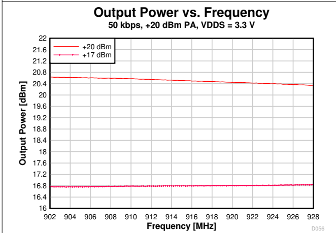
图 7-49. Output Power vs. Frequency (50 kbps, 915 MHz, VDDS = 3.3 V)
