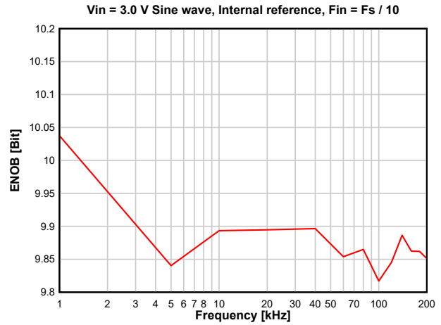
图 8-22. ENOB versus Sampling Frequency
