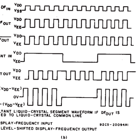
Fig. 17 - Display-driver circuit for one segment line and waveforms.
