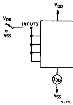
Fig. 12 - Quiescent-device-current test circuit.
