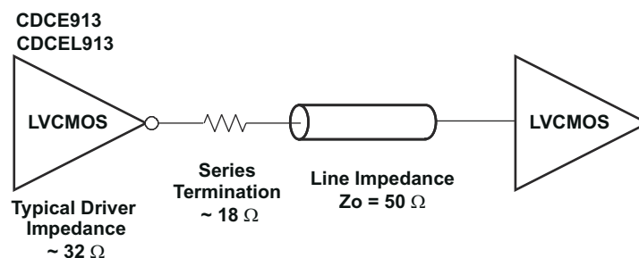
图 6-2. Test Load for 50- \Omega Board Environment
