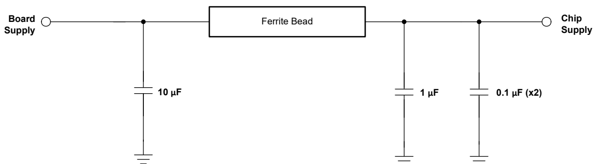
图 10-1. Power Supply Decoupling
