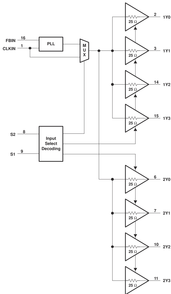
图 8-1. Functional Block Diagram
