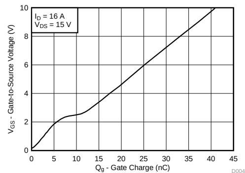
栅极电荷
