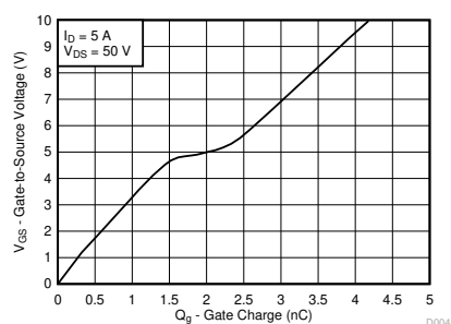
栅极电荷
