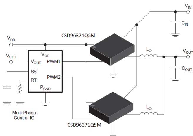
Figure 1. Application Diagram
